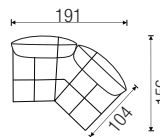
45 corner small without arm top view
