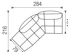
Terminal large L top view
